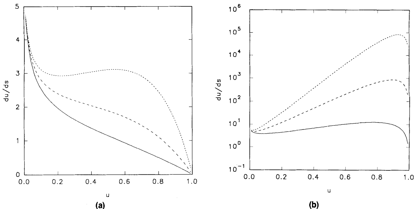
Figure 1. u_s vs. u for various values of M according to Eq. 5.
