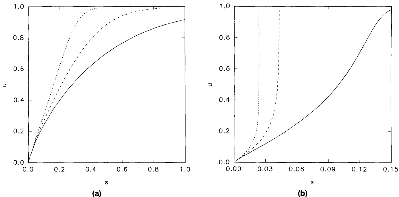
Figure 2. u vs. s for various values of M according to Eq. 10; the lower limit in Eq. 10 was set to 10^{-4} to avoid numerical overflow.
